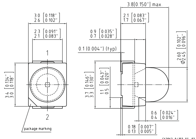
Figure 42: MULTILED
