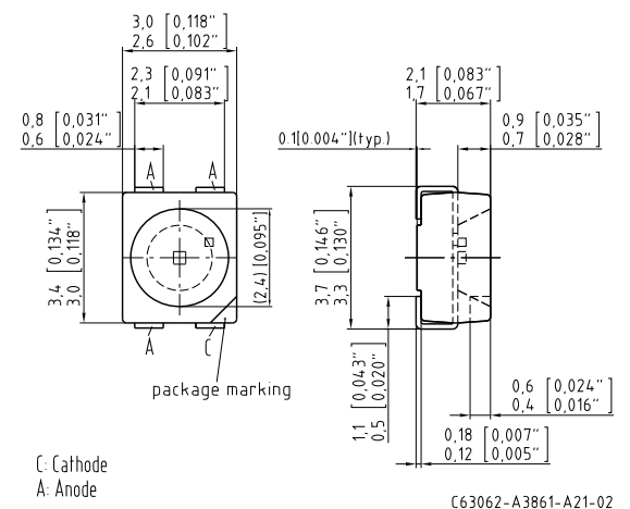
Figure 12: Power TOPLED
