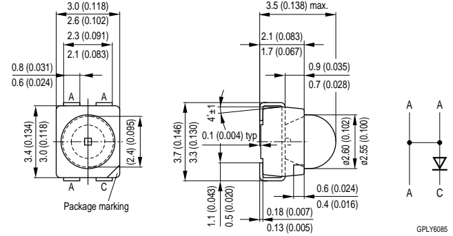
Figure 16: Multi TOPLED
