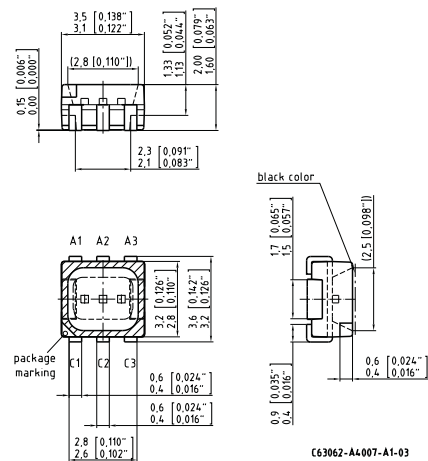
Figure 42: MULTILED
